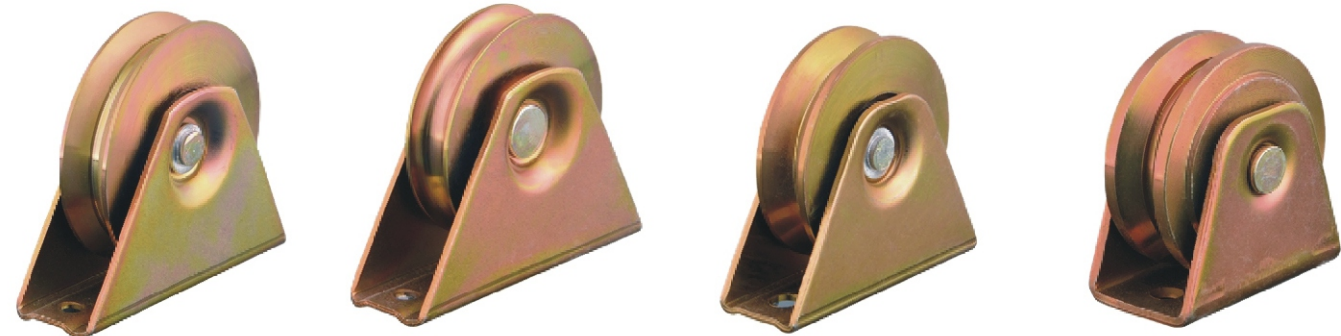
Single bearing, Y Groove GD-HA1Y50 50mm GD-HA1Y60 60mm GD-HA1Y70 70mm GD-HA1Y80 80mm GD-HA1Y90 90mm GD-HA1Y100 100mm Single bearing, U Groove GD-HA1U50 50mm GD-HA1U60 60mm GD-HA1U70 70mm GD-HA1U80 80mm GD-HA1U90 90mm GD-HA1U100 100mm Single bearing, V Groove GD-HA1V50 50mm GD-HA1V60 60mm GD-HA1V70 70mm GD-HA1V80 80mm GD-HA1V90 90mm GD-HA1V100 100mm Africa type Y/U/V groove can be choosen 45mm 80mm 60mm 100mm 70mm
