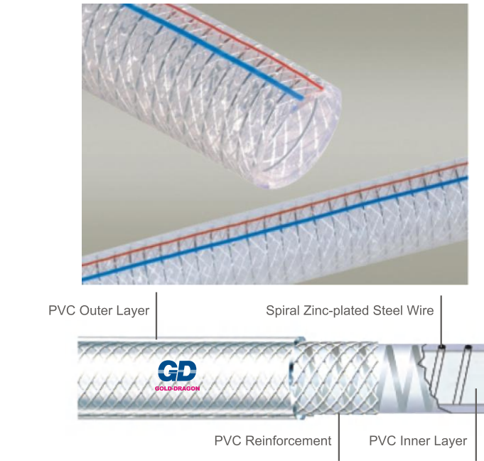
The regular specification of PVC fiber and steel wire reinforced hose
